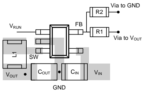
APW7507 Layout Suggestion
