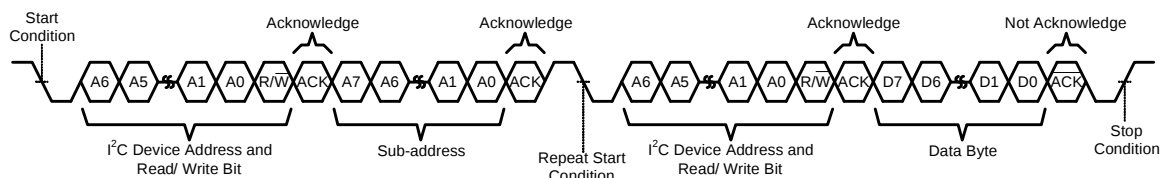
Figure 3. Single-Byte Read Transfer
