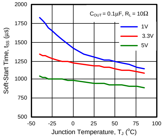
Soft-Start Time vs. Junction Temperature
