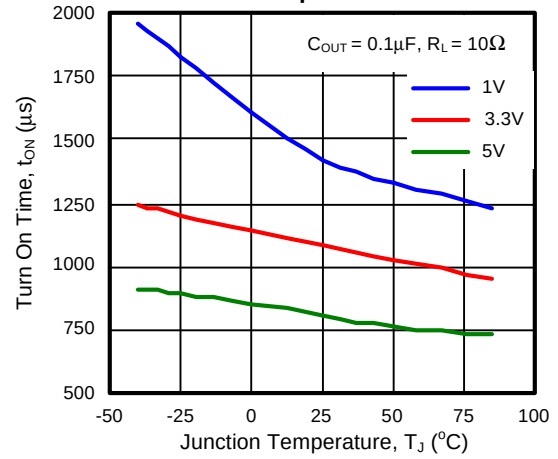
Turn On Time vs. Junction Temperature
