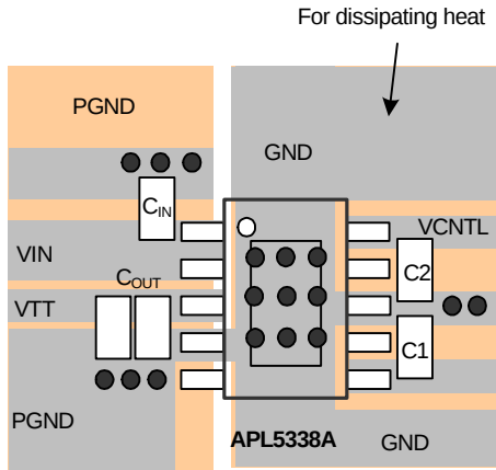
Figure 2. Recommended Layout
