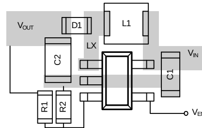
Optimized APW7137 Layout
