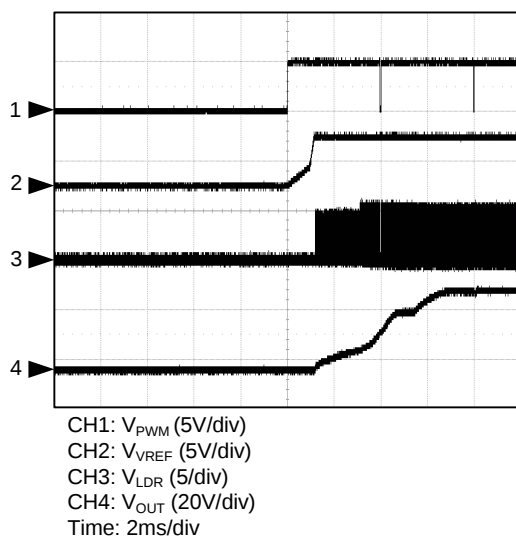
PWM Dimming Enable, 250Hz, 99%
