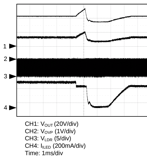
One String Open
