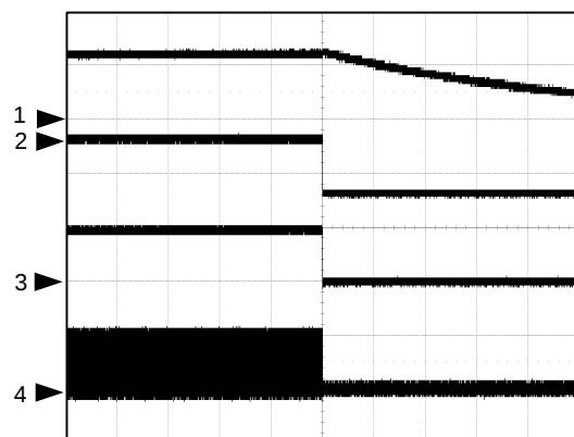
Over-Temperature Protection
