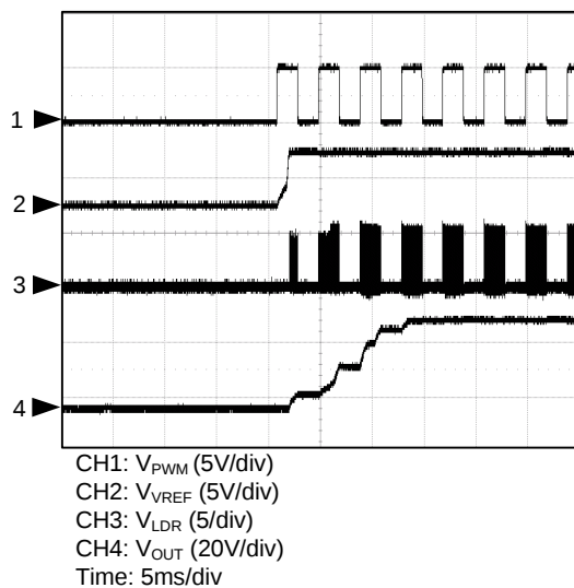
PWM Dimming Enable, 250Hz, 50%
