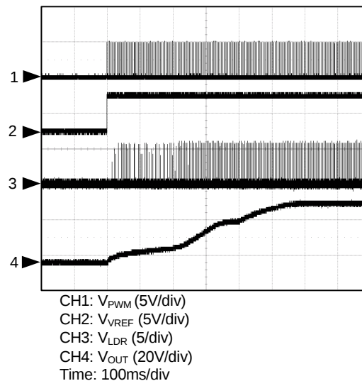
PWM Dimming Enable, 250Hz, 1%
