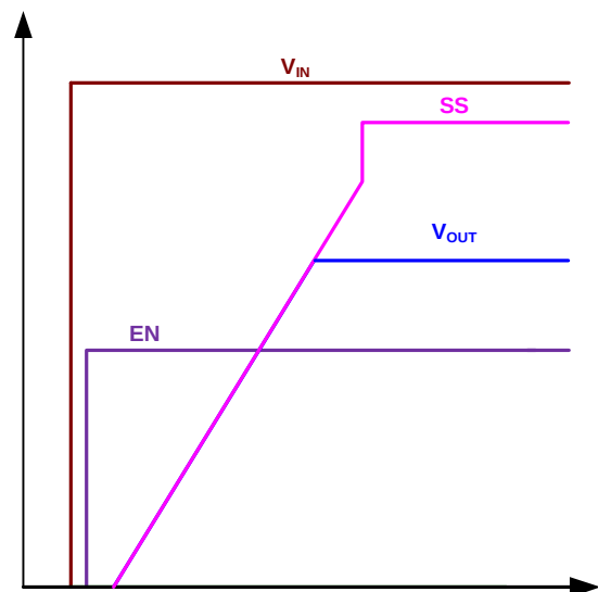
Figure 1. Soft-Start Sequence
