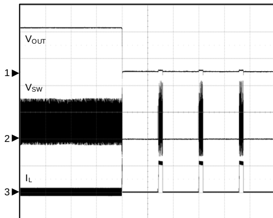
Short-Current Entry
