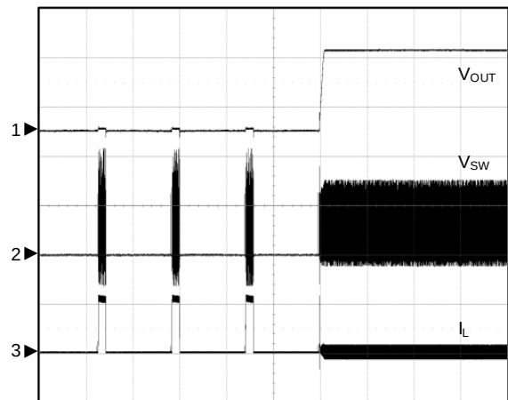
Short-Current Recovery
