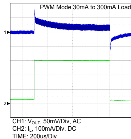
Figure 9. PWM Mode 30mA to 300mA Load Transient
