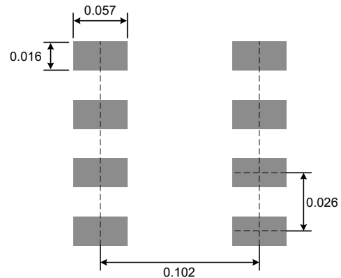
Figure 16. TSOT-23-8A Minimum Footprint
