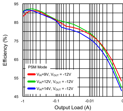
Figure 7. Efficiency
