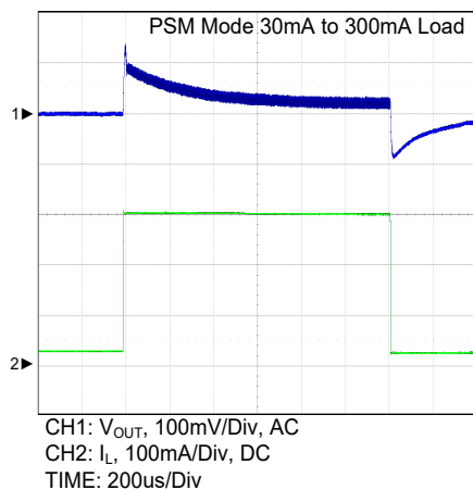
Figure 8. PSM Mode 30mA to 300mA Load Transient
