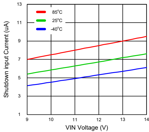
Figure 3. Shutdown Current
