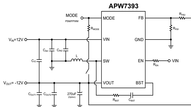
Figure 1. Application Circuit
