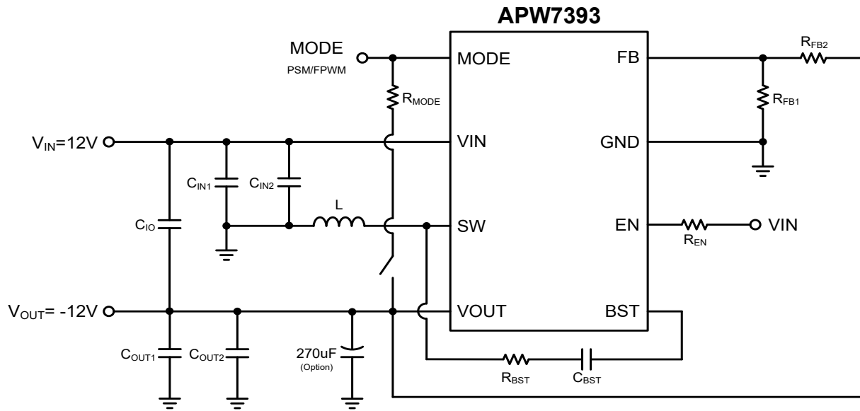
Figure 10. Application Circuit
