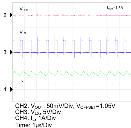
Steady State
