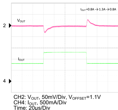
Load Transient
