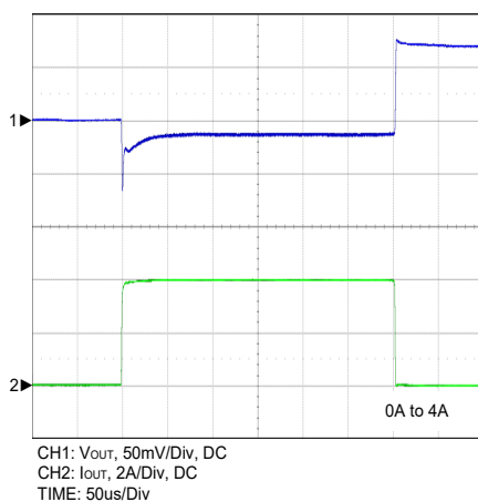
Figure 20. DCM to CCM Load Transient
