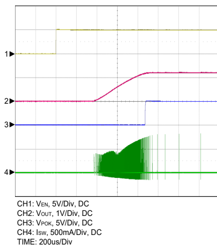
Figure 14. EN Power On Without Output Loading
