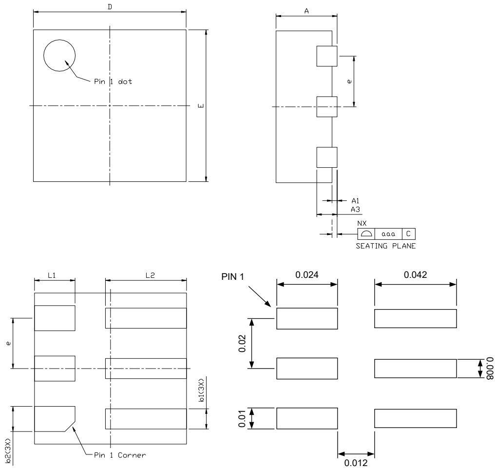
Recommended Land Pattern unit : inch
