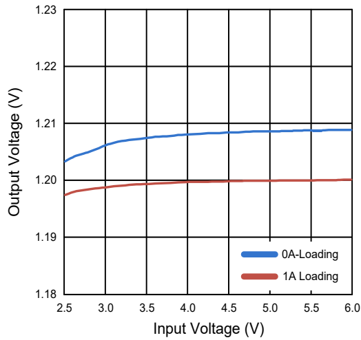
Figure 1. Output Voltage vs. Input Voltage
