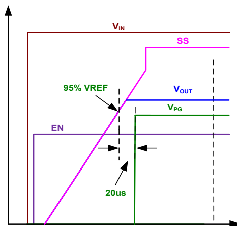
Figure 24. Soft-Start Sequence
