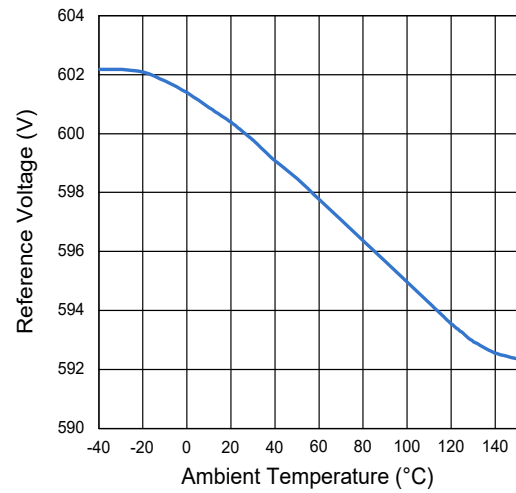
Figure 4. Reference Voltage vs. Ambient Temperature
