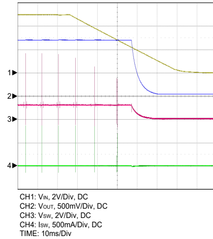
Figure 11. VIN Power Off Without Output Loading
