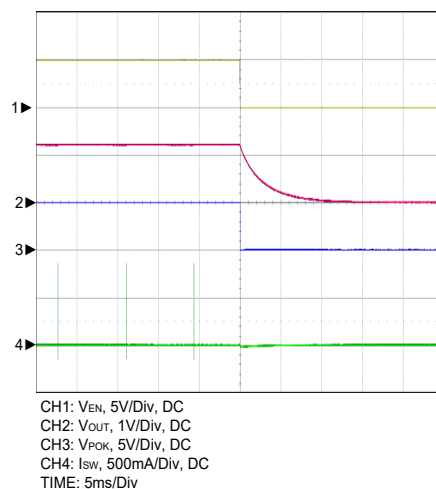
Figure 15. EN Power Off Without Output Loading
