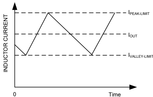
Figure 25. Current Limit Algorithm
