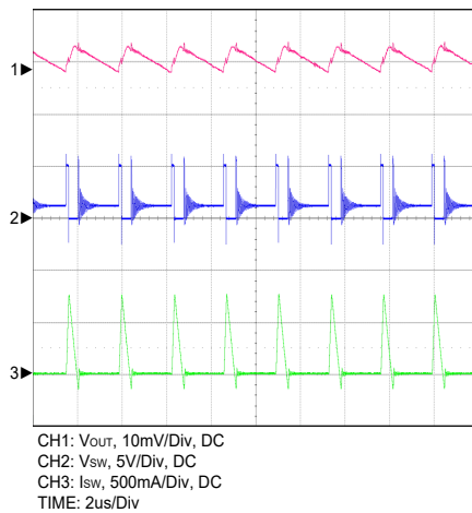
Figure 18. Normal Operation In Light Load
