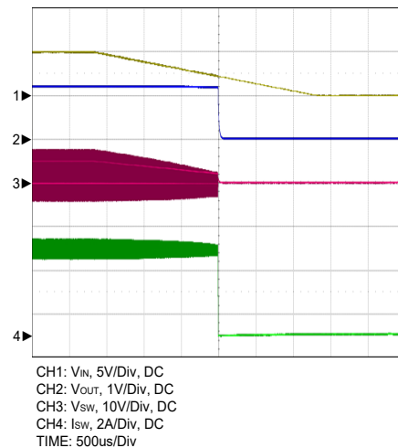
Figure 13. VIN Power Off With Output Loading
