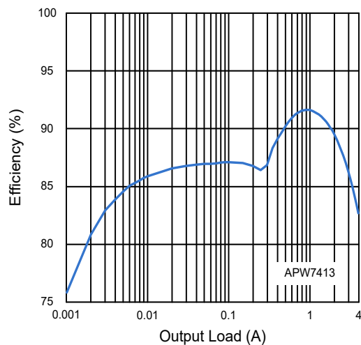
Figure 9. Efficiency
