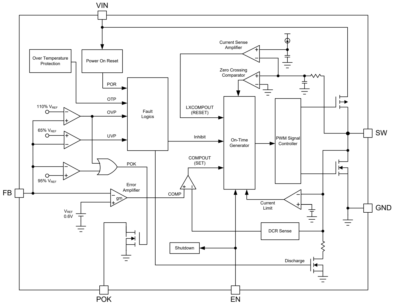
Figure 23. Function Block Diagram
