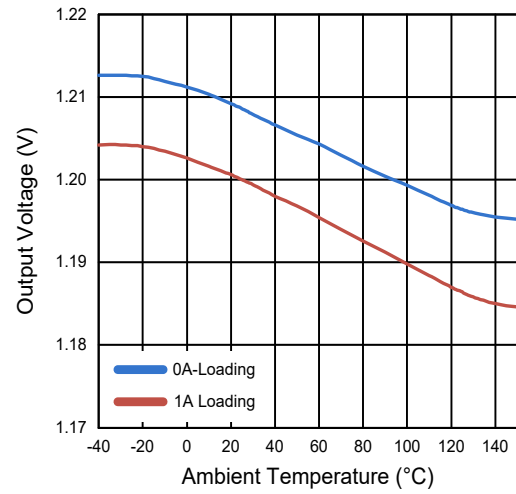
Figure 2. Output Voltage vs. Ambient Temperature
