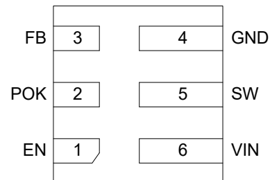
DFN / VTDFN Package 6-Pin Bottom View
