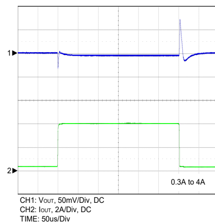
Figure 21. CCM to CCM Load Transient
