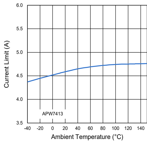
Figure 8. Low-Side Current Limit vs. Ambient Temperature
