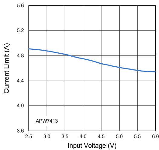
Figure 7. Low-Side Current Limit vs. Input Voltage
