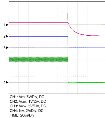
Figure 17. EN Power Off With Output Loading
