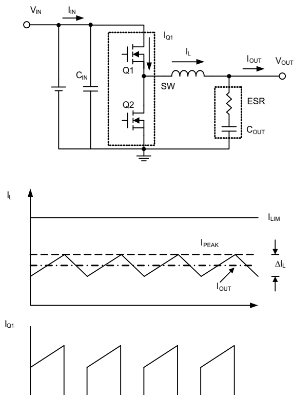
Figure 27. Buck Converter Application Information
