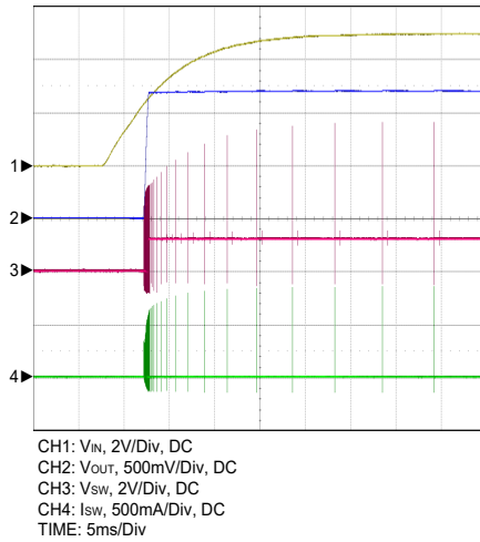
Figure 10. VIN Power On Without Output Loading
