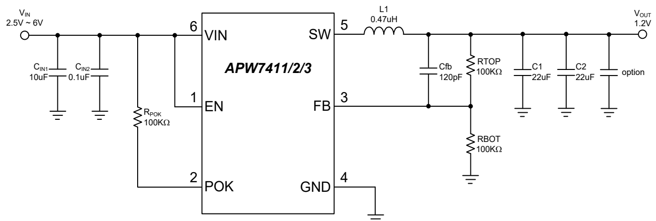
Figure 22. Typical Application Circuit of APW7411/2/3
