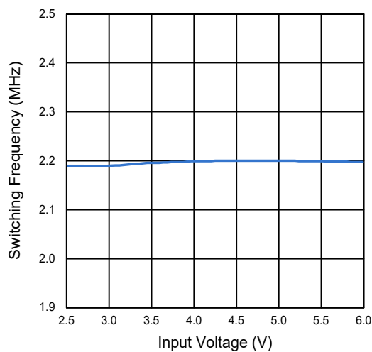
Figure 5. Switching Frequency vs. Input Voltage
