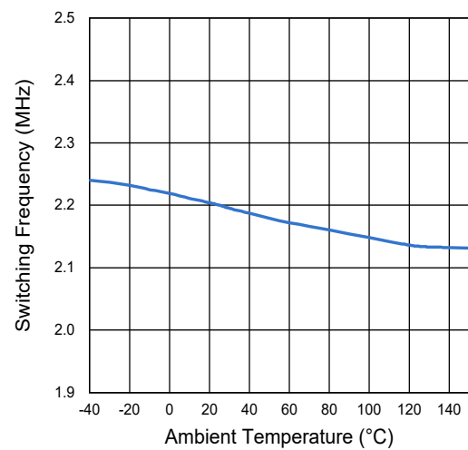
Figure 6. Switching Frequency vs. Ambient Temperature
