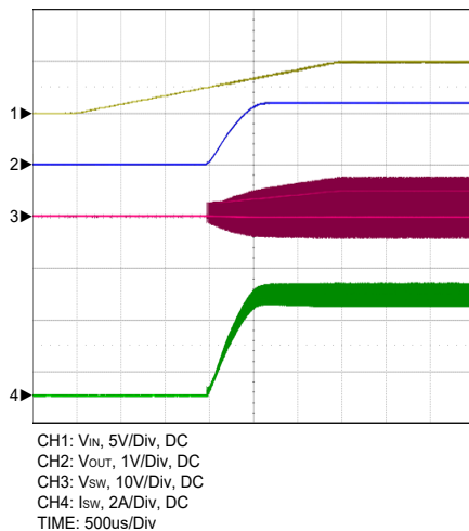
Figure 12. VIN Power On With Output Loading
