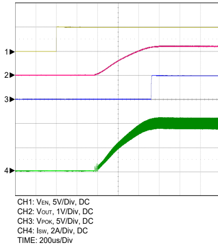
Figure 16. EN Power On With Output Loading
