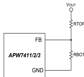
Figure 26. Output Voltage Setting
