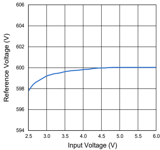
Figure 3. Reference Voltage vs. Input Voltage
