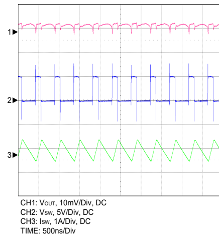
Figure 19. Normal Operation In Heavy Load
