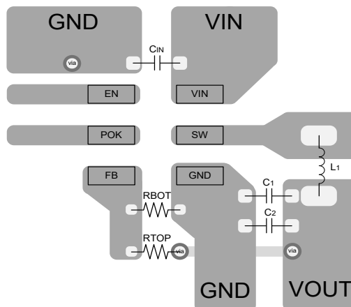
Figure 28. PCB Layout Recommendation
