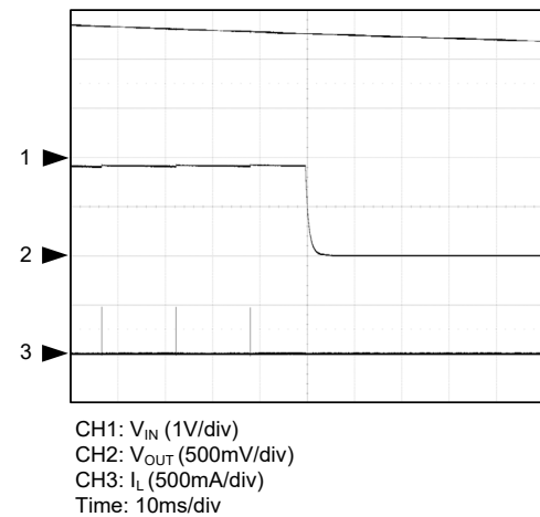
Power Off VIN with Discharge
