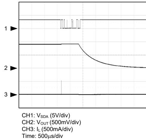
Shutdown by I2C with Discharge
