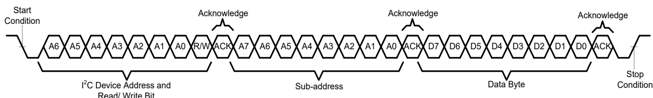
Figure 2. Single-Byte Write Transfer
