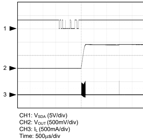
Enabled by I2C
