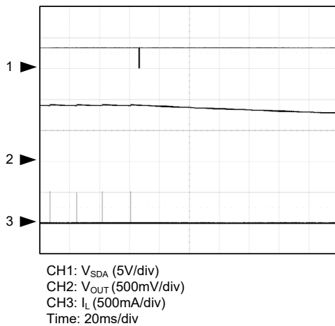
Shutdown by I2C with No Discharge
