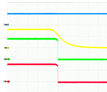
VIN Power Down With Loading
