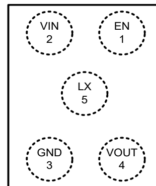
WLCSP 0.90x0.74-5
