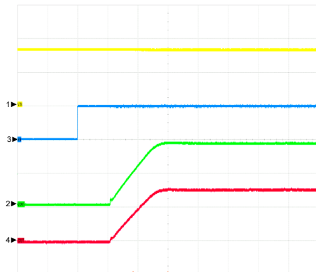
Enable With Loading
