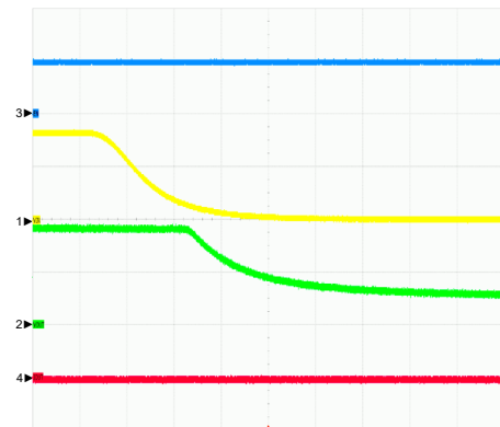
VIN Power Down Without Loading
