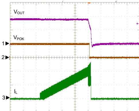
Current Limit
