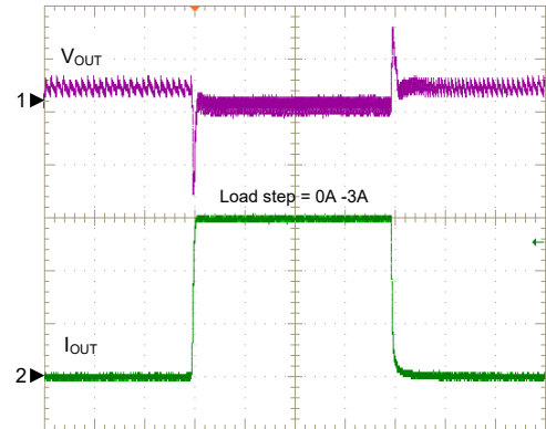
Load Transient
