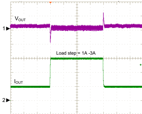
Load Transient
