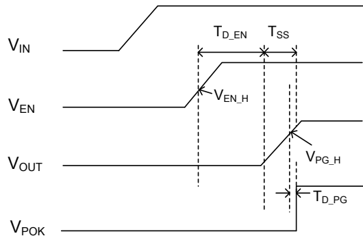
Figure 1. APW8827A Power On Sequence
