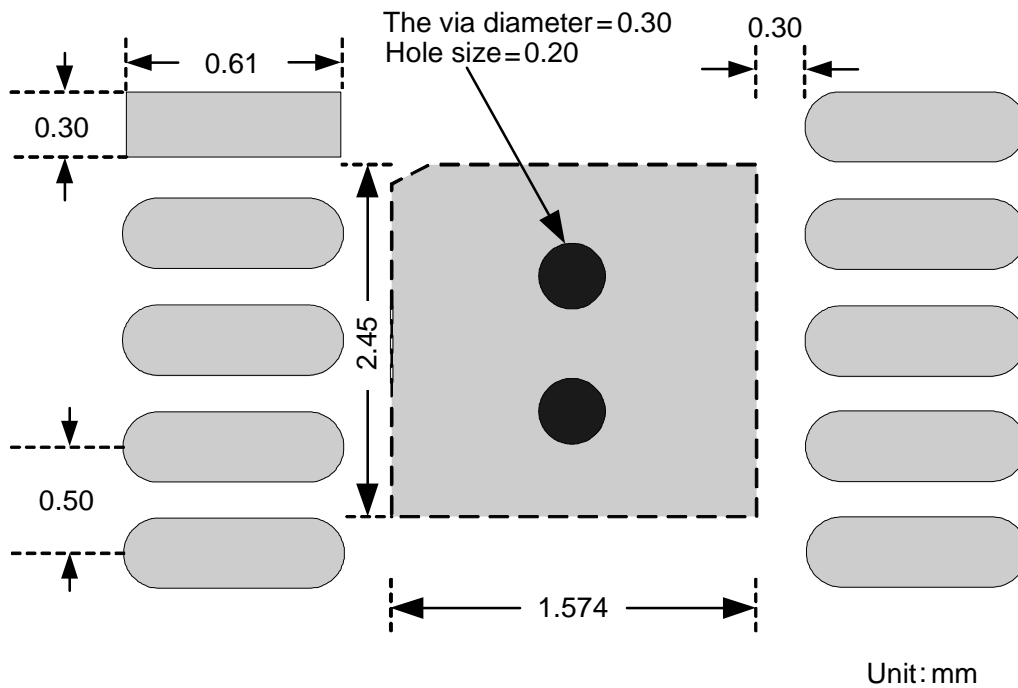
TDFN3x3-10 Land Pattern Recommendation
