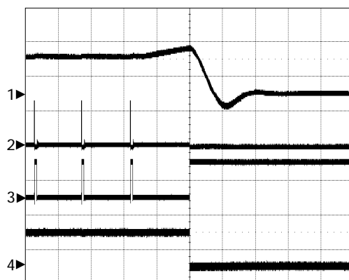
Over-Voltage Protection
