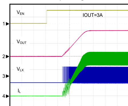
Start Up through V_{EN}
