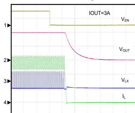
Shut Down through V_{EN}
