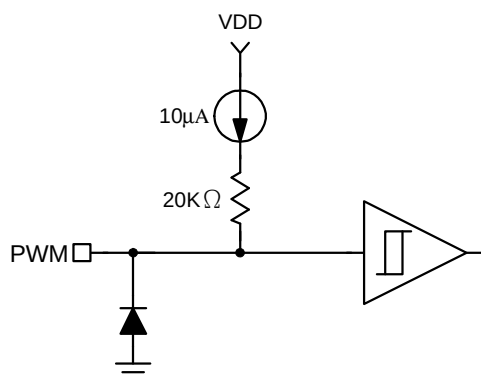
(3) PWM speed control input pin (PWM)
