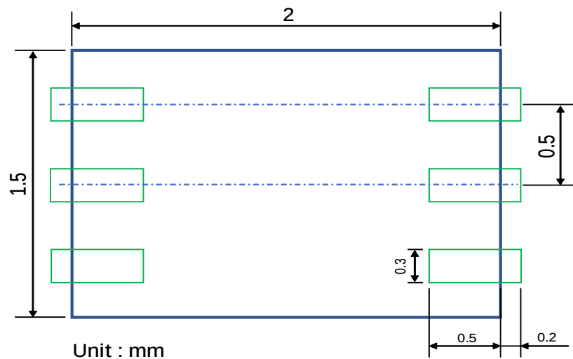
Recommended Minimum Footprint
