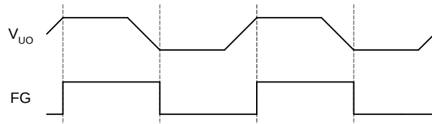
Figure 3. FG Output Waveform
