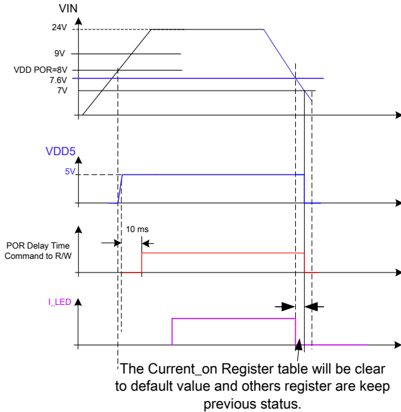
Figure 1: Power Sequence
