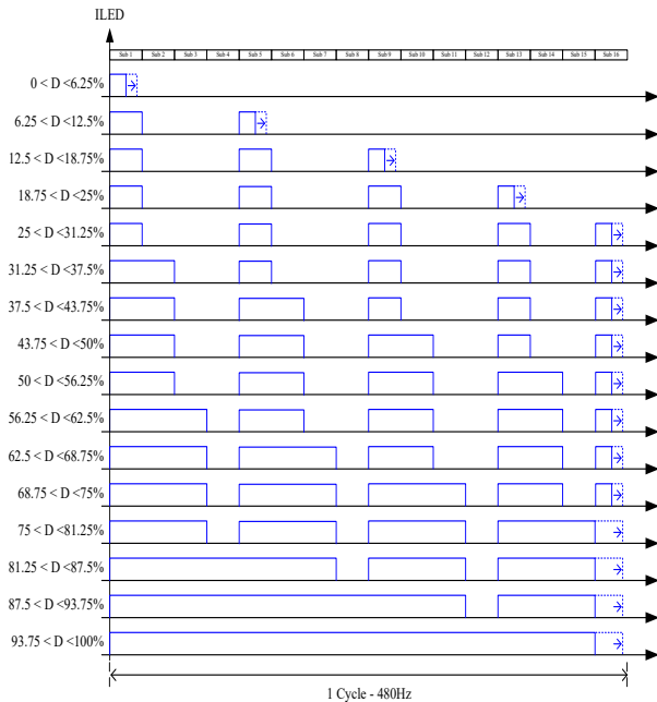
Figure 6: LED current of PFM mode
