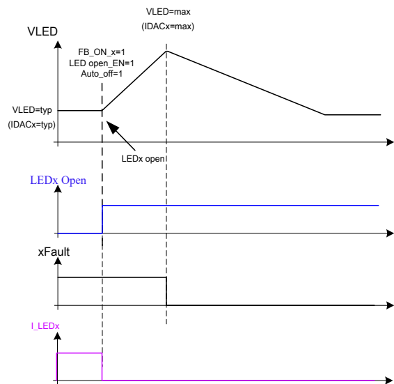
Figure 2: LED open - auto off
