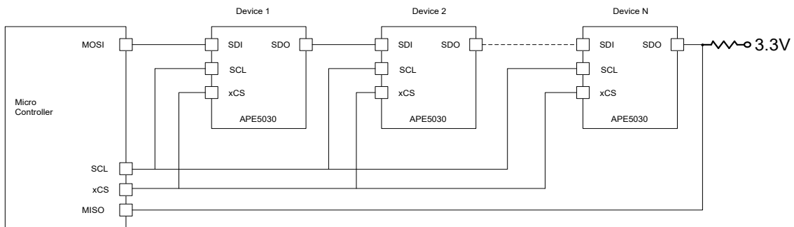
Figure 7: SPI Daisy Chain structure
