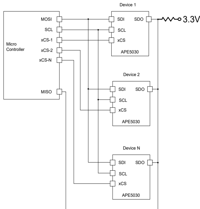
Figure 8: SPI Parallel Structure
