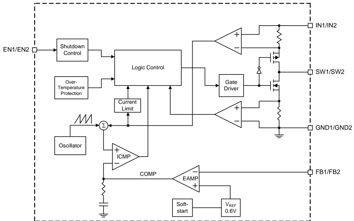
Diagram Represents 1/2 of the APW7179
