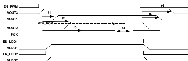
Figure 1. Power sequence
