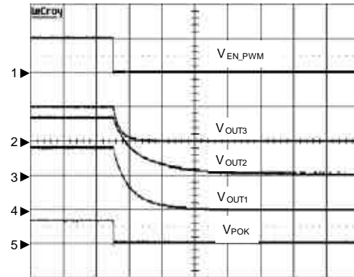
Turn Off Response -PWM Converter
