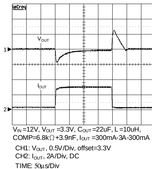
Load Transient
