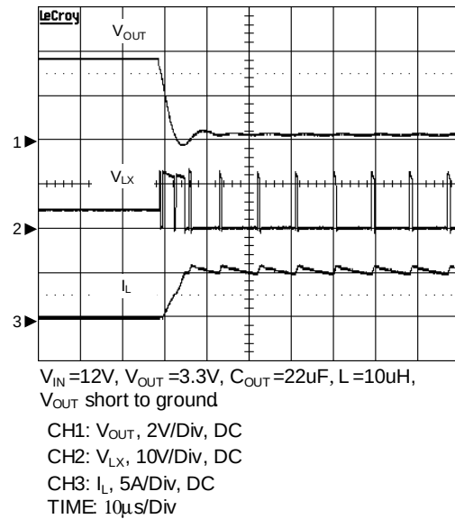
Short Circuit
