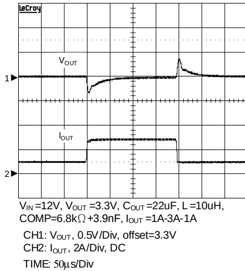
Load Transient
