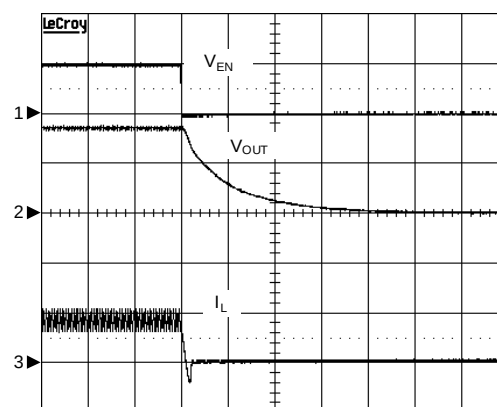
Shutdown
