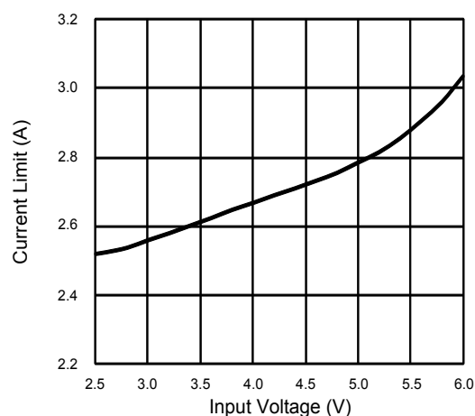
Figure 6. Current Limit vs. Input Voltage
