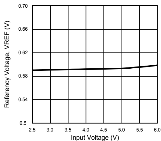
Figure 2. Reference Voltage vs. Input Voltage
