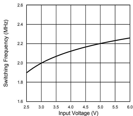
Figure 4. Switching Frequency vs. Input Voltage
