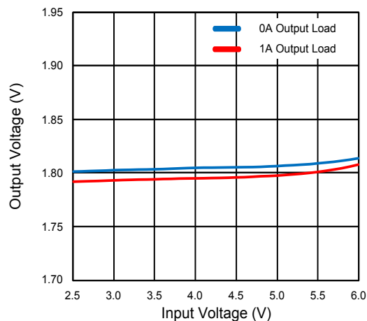
Figure 10. Line Regulation
