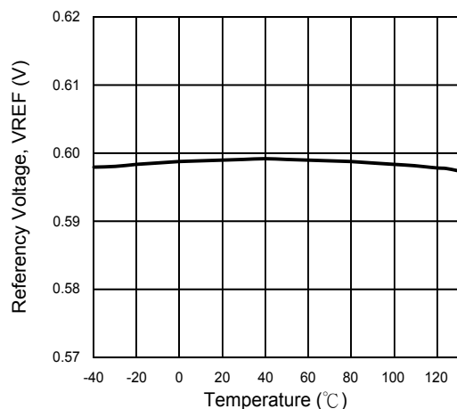
Figure 1. Reference Voltage vs. Temperature
