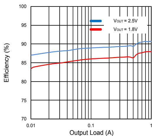
Figure 11. Efficiency
