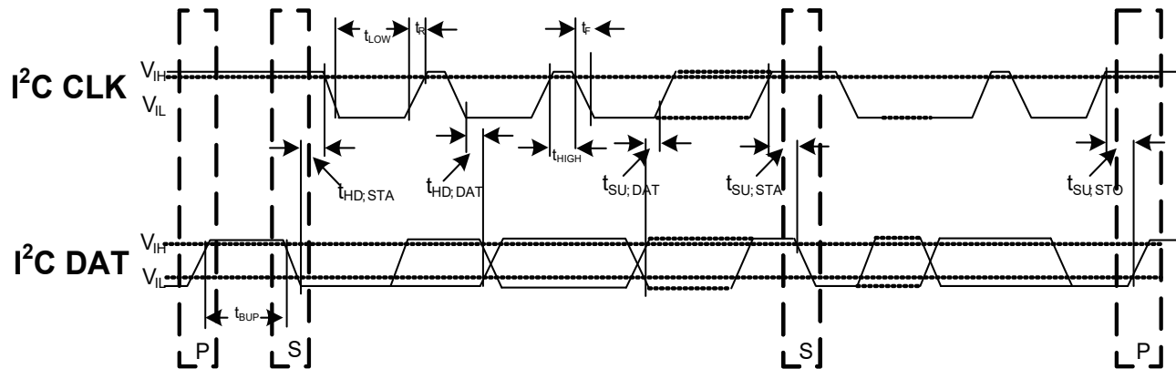
Figure 4: SMBus Common AC Specification
