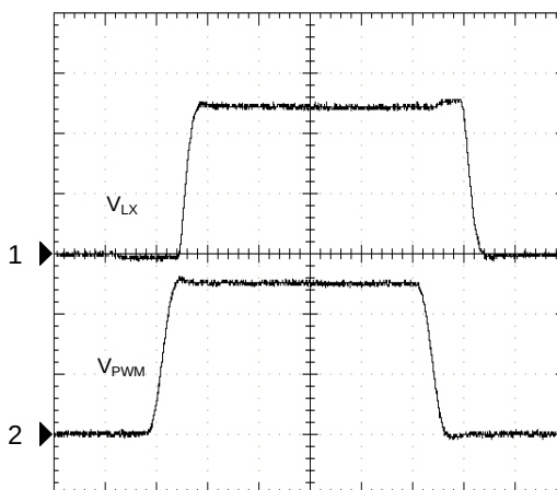
PWM Operation
