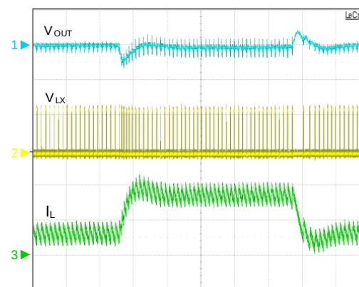
Load Transient 2
