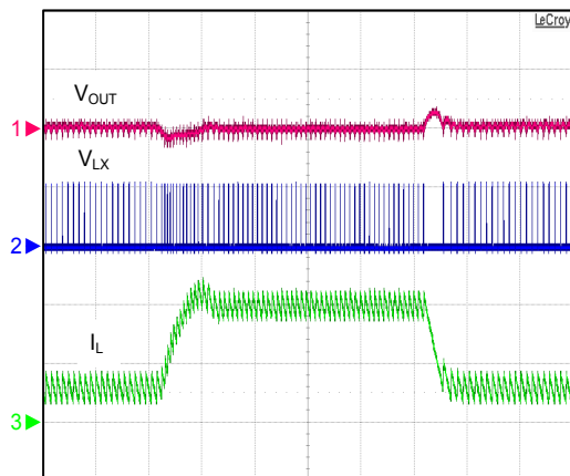
Load Transient
