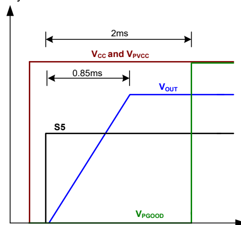
Fig1. Soft-Start Sequence
