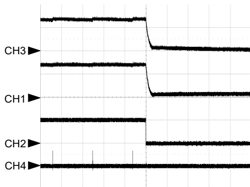
Disable S3/S5 - No Load
