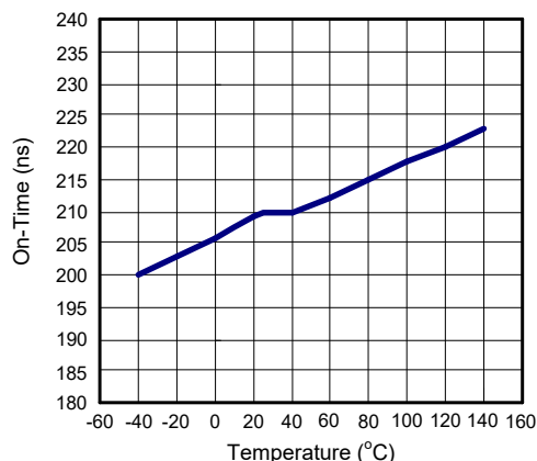
On-Time VS Temperature
