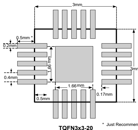
Figure3. Recommended Minimum Footprint
