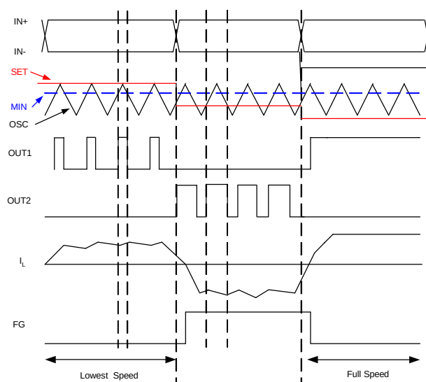
Figure 1. Rotation Waveform
