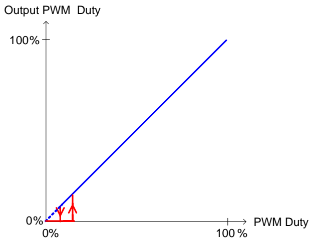
Figure 4. PWM mode
