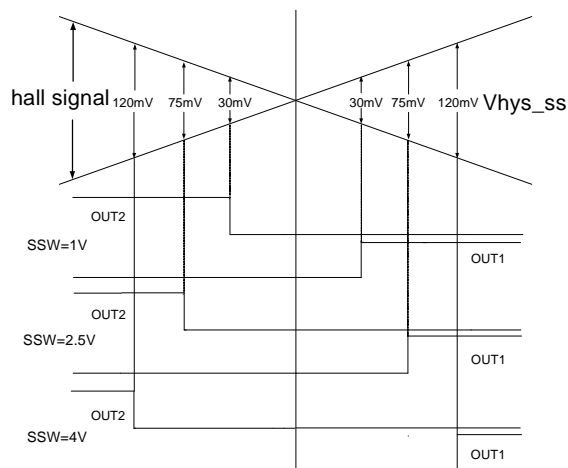
Figure 6. When hall signal > V hys_ss .
