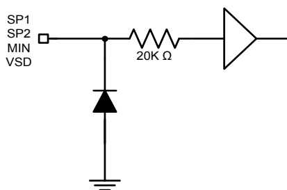
(9) Input and output duty setting input pin (SP1,SP2,MIN,VSD)
