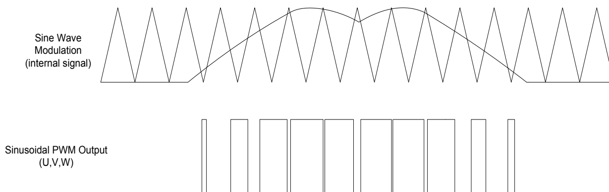
Figure 7: Sine Wave Modulation PWM Output
