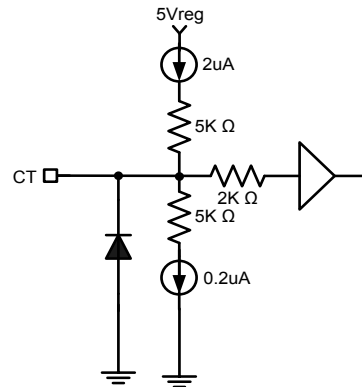
(14) CT setting input pin (CT)
