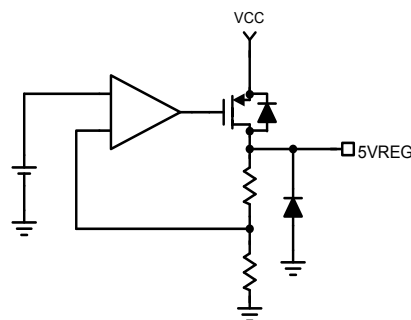
(2) Regulator output pin (5VREG)
