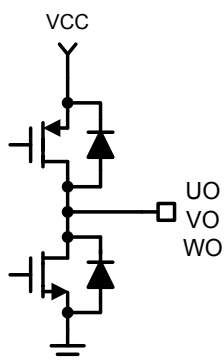
(5) Driver output pin (UO, VO, WO)
