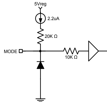
(16) MODE setting input pin (MODE)
