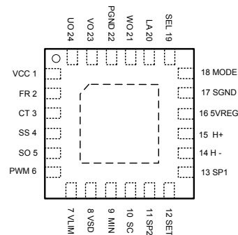
QFN4x4-24A Top View
