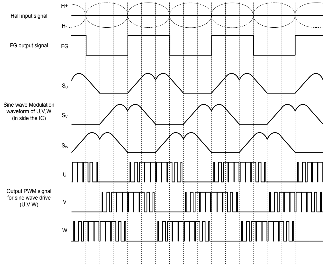
Figure 6: Reverse Rotation Input and Output timing chards
