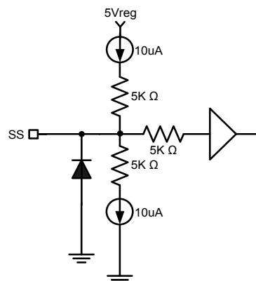
(8) Soft -Start Time setting input pin (SS)
