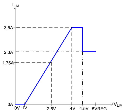
Figure8: Current Limit Control
