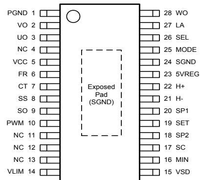
TSSOP-28P
