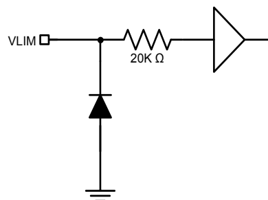
(10) Current Limit setting input pin (VLIM )
