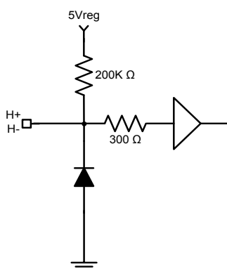
(3) Hall signal input pin (H+, H-)
