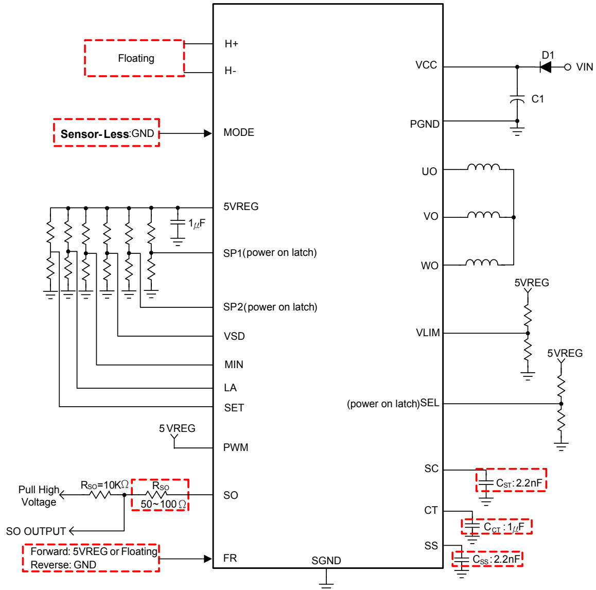
Circuit 4: SET Voltage Input Speed Control For Sensor-Less
