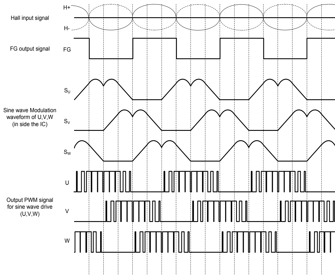
Figure 5: Forward Rotation Input and Output timing chards
