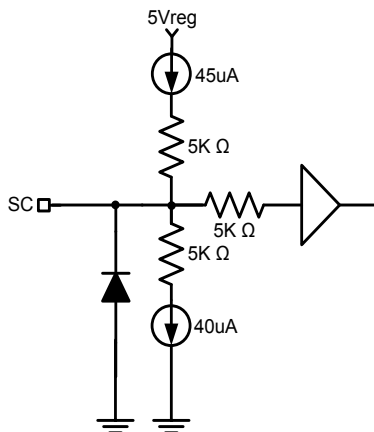
(15) Start- up Time setting input pin (SC)
