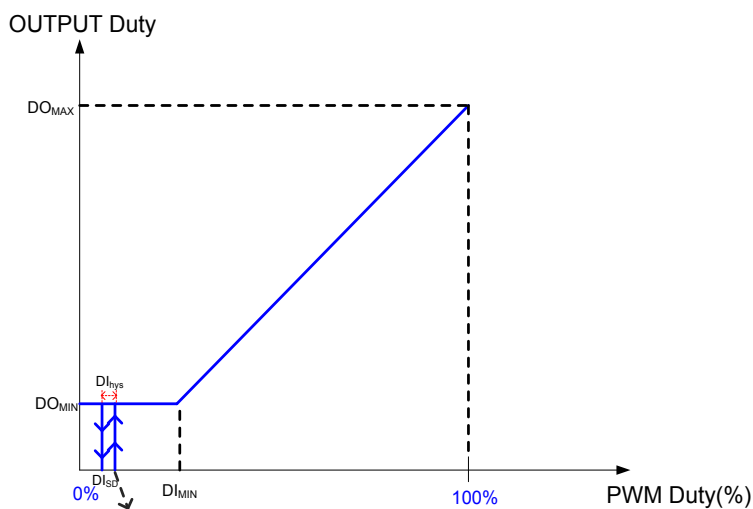
Figure1: Output Duty Control
