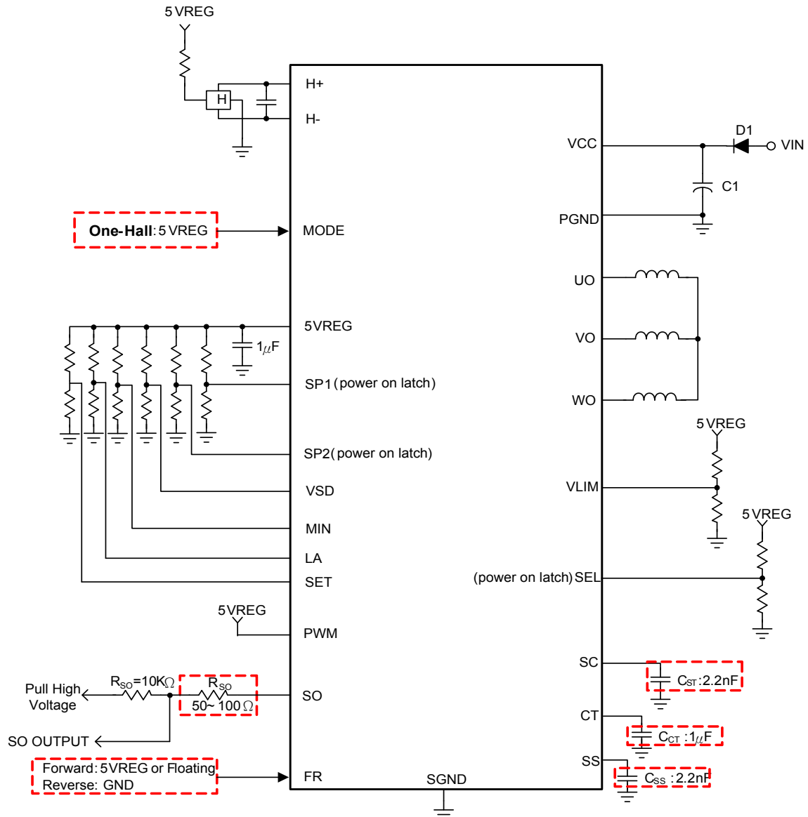
Circuit 2: SET Voltage Input Speed Control For One-Hall
