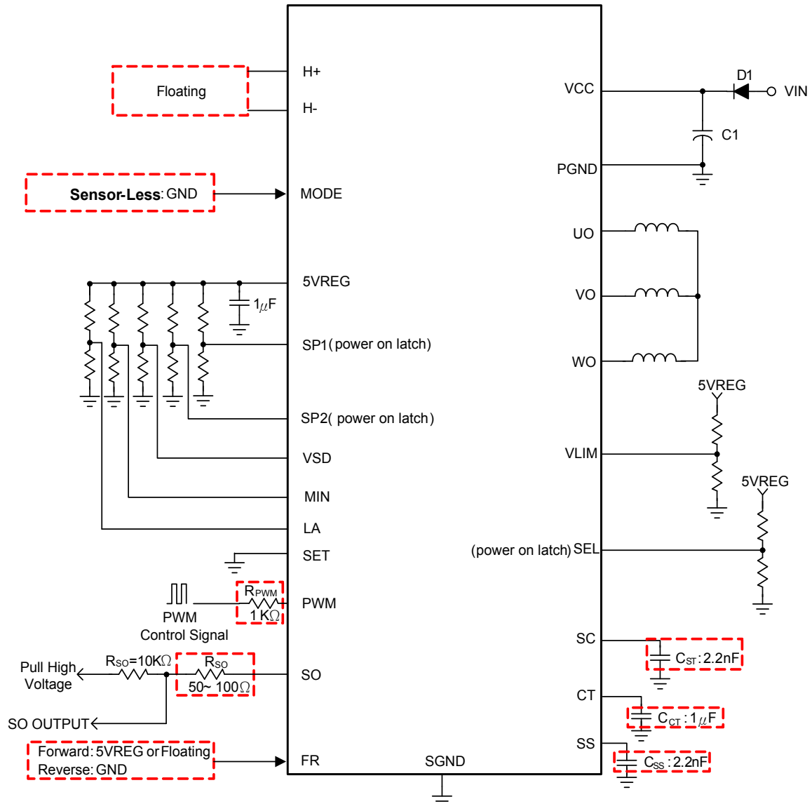
Circuit 3: PWM Speed Control For Sensor-Less
