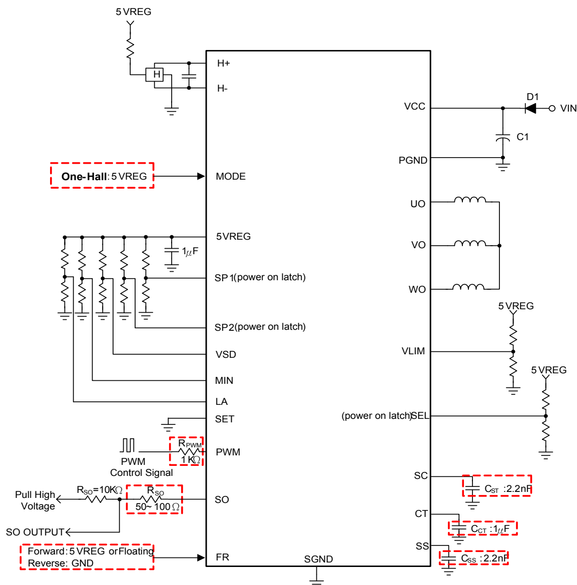
Circuit 1: PWM Speed Control For One-Hall
