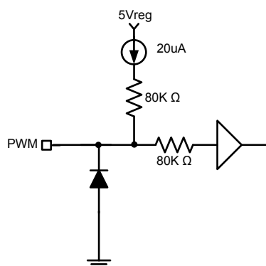
(7) PWM speed control input pin (PWM)
