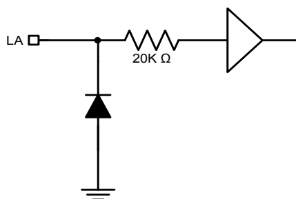
(11) Lead Angle setting input pin (LA )
