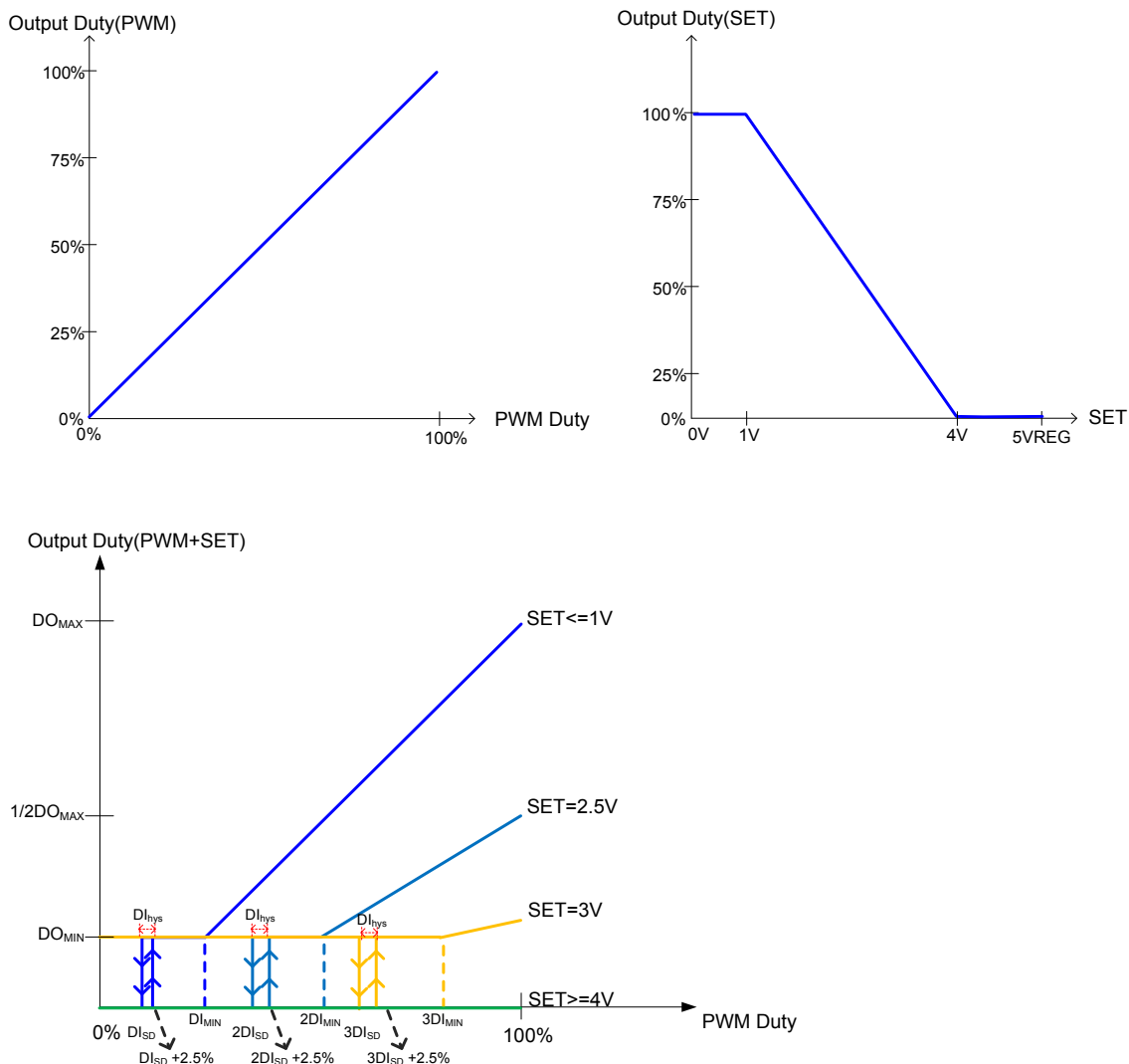
Figure3: Direct PWM Mode or SET Mode or PWM+SET Mode Output Duty Control
