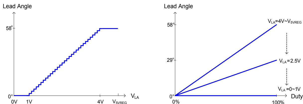
Figure4: Lead Angle Control
